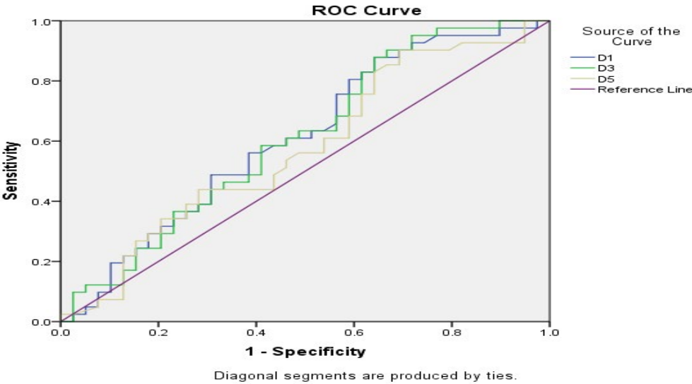
Figure 1: ROC curve.
