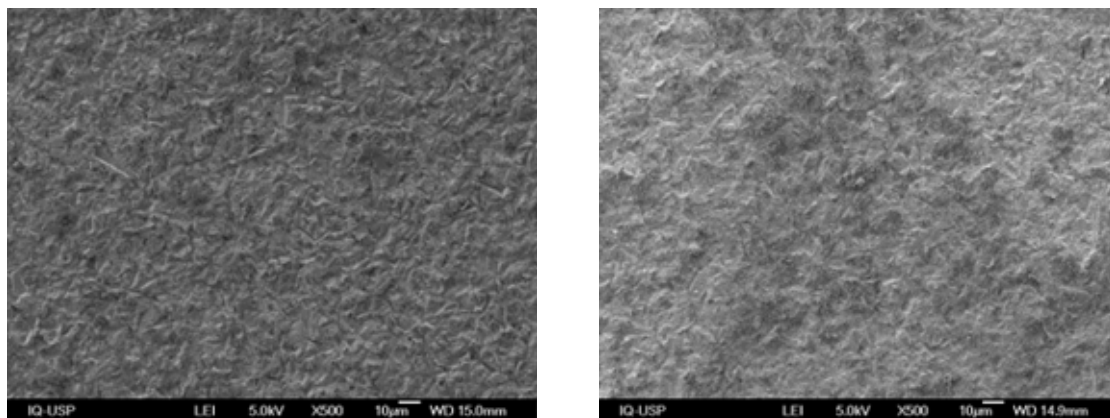
Figure 3: In A and B surfaces of Titanium and Zirconia (Y-TZP), respectively, after microblasting with silicic acid-modified aluminum oxide (SMAO).
